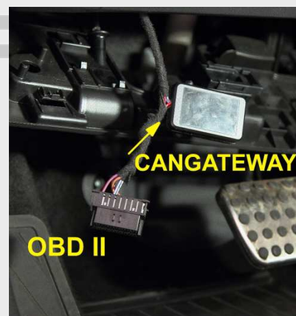
CANGATEWAY OBDII in the car
